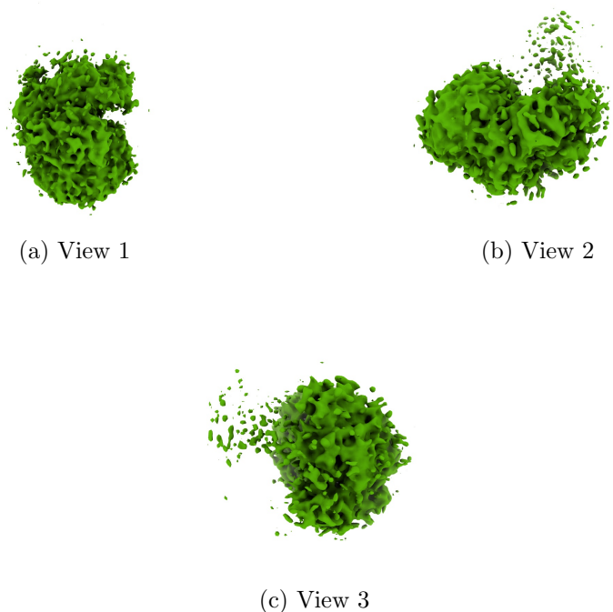
Figure 4: Isosurface at threshold=0.402000. Views generated by ChimeraX at a the following X, Y, Z angles: View 1 (0, -90, -90), View 2 (-90, 0, -90), View 3 (0, 0, 0).
