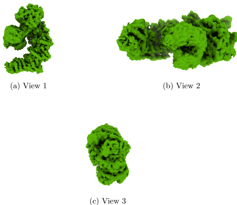
Figure 4: Isosurface at threshold=0.334000. Views generated by ChimeraX at a the following X, Y, Z angles: View 1 (0, -90, -90), View 2 (-90, 0, -90), View 3 (0, 0, 0).
