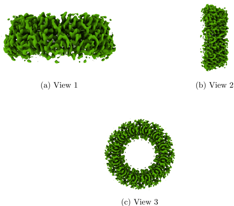
Figure 4: Isosurface at threshold=1.600000. Views generated by ChimeraX at a the following X, Y, Z angles: View 1 (0, -90, -90), View 2 (-90, 0, -90), View 3 (0, 0, 0).
