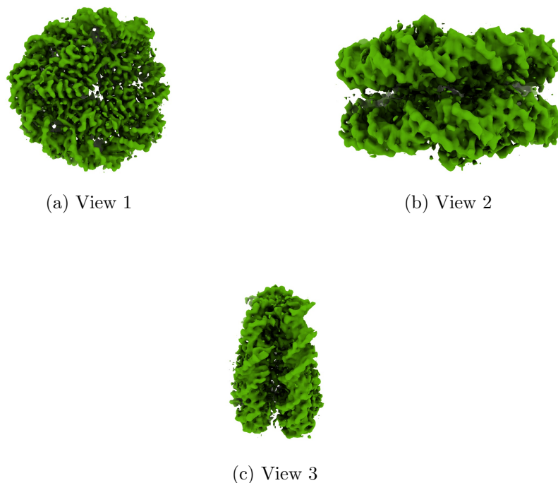
Figure 4: Isosurface at threshold=0.200000. Views generated by ChimeraX at the following X, Y, Z angles: View 1 (0, -90, -90), View 2 (-90, 0, -90), View 3 (0, 0, 0).
