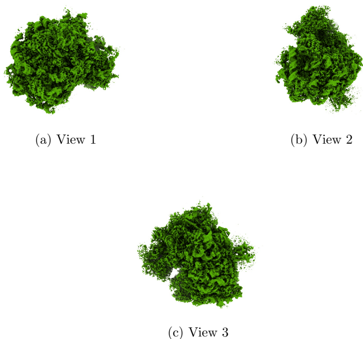
Figure 4: Isosurface at threshold=0.023100. Views generated by ChimeraX at a the following X, Y, Z angles: View 1 (0, -90, -90), View 2 (-90, 0, -90), View 3 (0, 0, 0).
