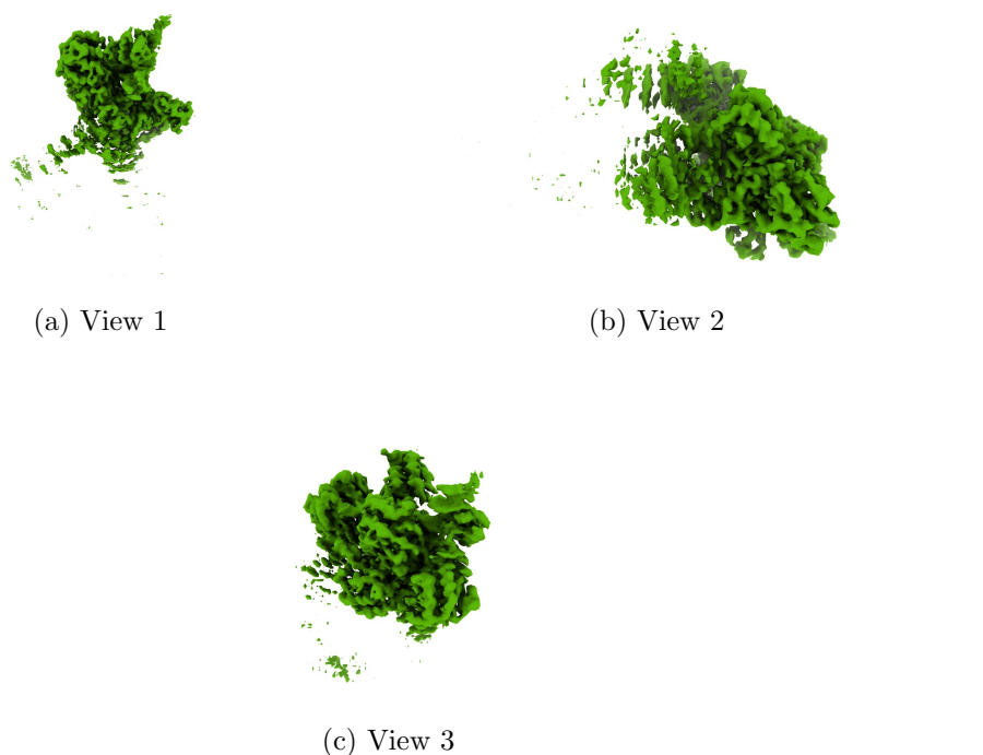
Figure 4: Isosurface at threshold=0.350000. Views generated by ChimeraX at a the following X, Y, Z angles: View 1 (0, -90, -90), View 2 (-90, 0, -90), View 3 (0, 0, 0).
