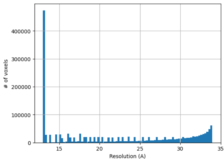
Figure 22: Histogram of the local resolution according to MonoRes.
