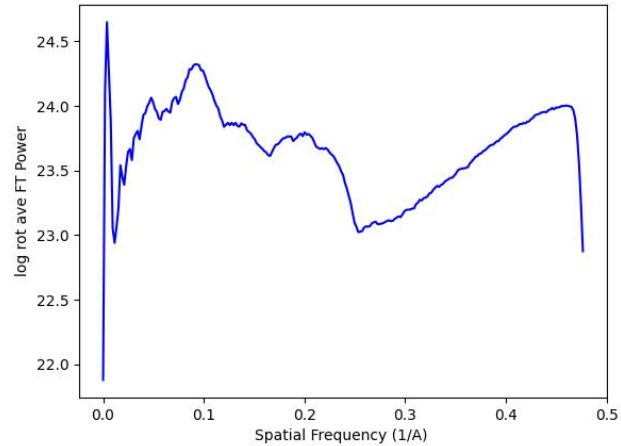
Figure 31: Logarithm of the radial average of the input map power in Fourier space.
