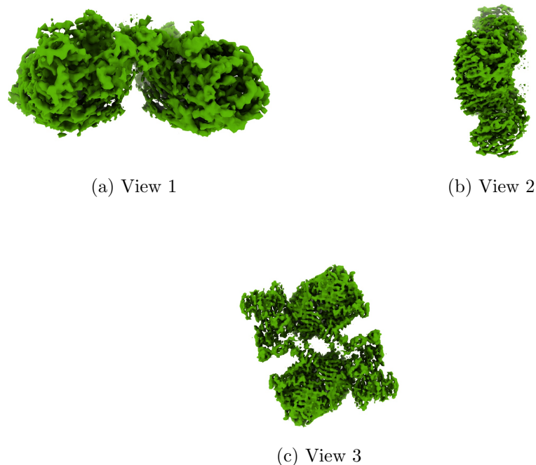
Figure 4: Isosurface at threshold=0.010400. Views generated by ChimeraX at a the following X, Y, Z angles: View 1 (0, -90, -90), View 2 (-90, 0, -90), View 3 (0, 0, 0).
