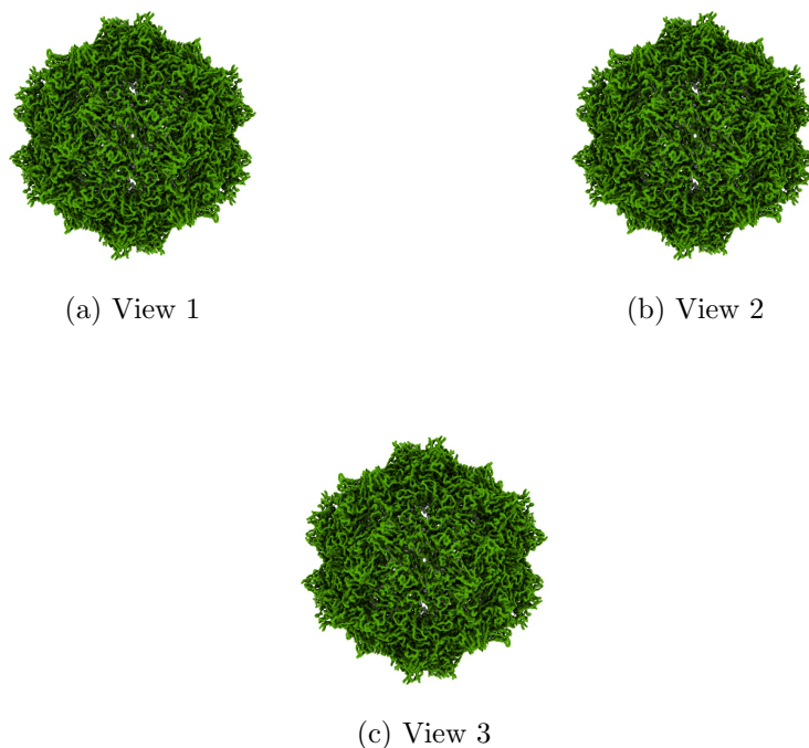
Figure 4: Isosurface at threshold=0.006910. Views generated by ChimeraX at a the following X, Y, Z angles: View 1 (0, -90, -90), View 2 (-90, 0, -90), View 3 (0, 0, 0).
