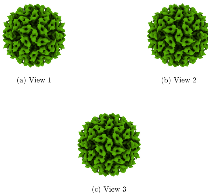
Figure 4: Isosurface at threshold=47.000000. Views generated by ChimeraX at a the following X, Y, Z angles: View 1 (0, -90, -90), View 2 (-90, 0, -90), View 3 (0, 0, 0).
