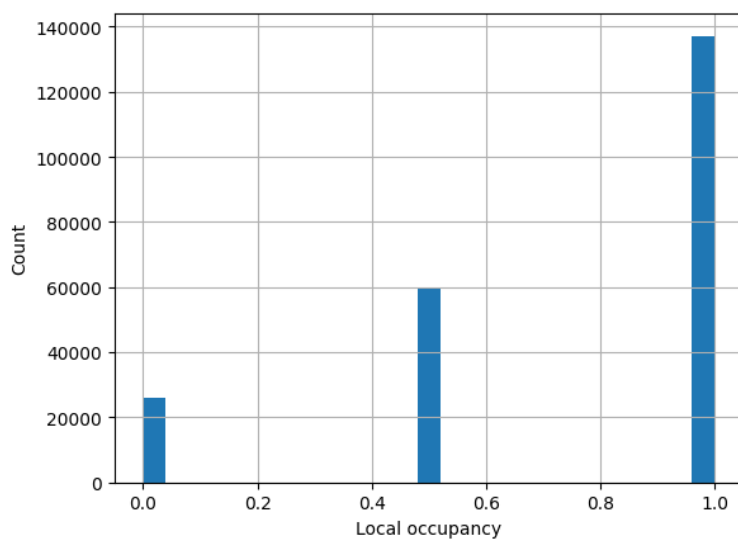
Figure 10: Histogram of the local occupancy according to LocOccupancy.
