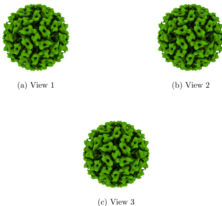
Figure 4: Isosurface at threshold=43.000000. Views generated by ChimeraX at a the following X, Y, Z angles: View 1 (0, -90, -90), View 2 (-90, 0, -90), View 3 (0, 0, 0).
