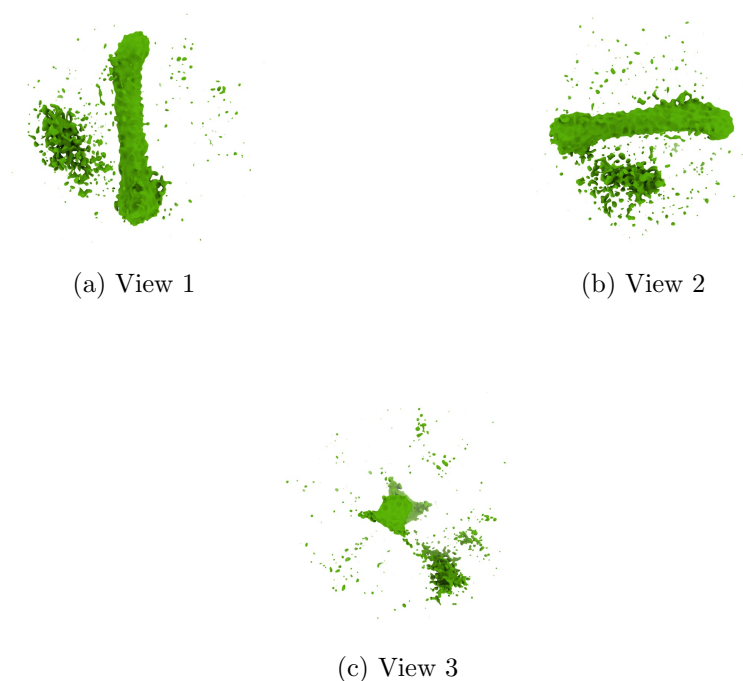
Figure 4: Isosurface at threshold=0.007410. Views generated by ChimeraX at a the following X, Y, Z angles: View 1 (0, -90, -90), View 2 (-90, 0, -90), View 3 (0, 0, 0).
