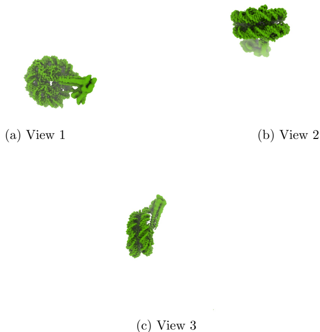
Figure 4: Isosurface at threshold=0.020000. Views generated by ChimeraX at a the following X, Y, Z angles: View 1 (0, -90, -90), View 2 (-90, 0, -90), View 3 (0, 0, 0).
