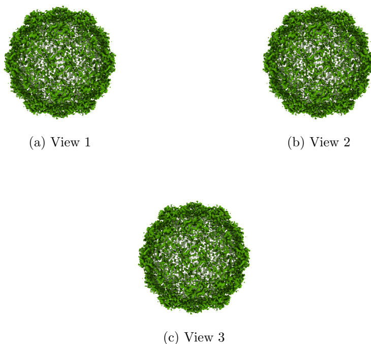
Figure 4: Isosurface at threshold=1.030000. Views generated by ChimeraX at a the following X, Y, Z angles: View 1 (0, -90, -90), View 2 (-90, 0, -90), View 3 (0, 0, 0).
