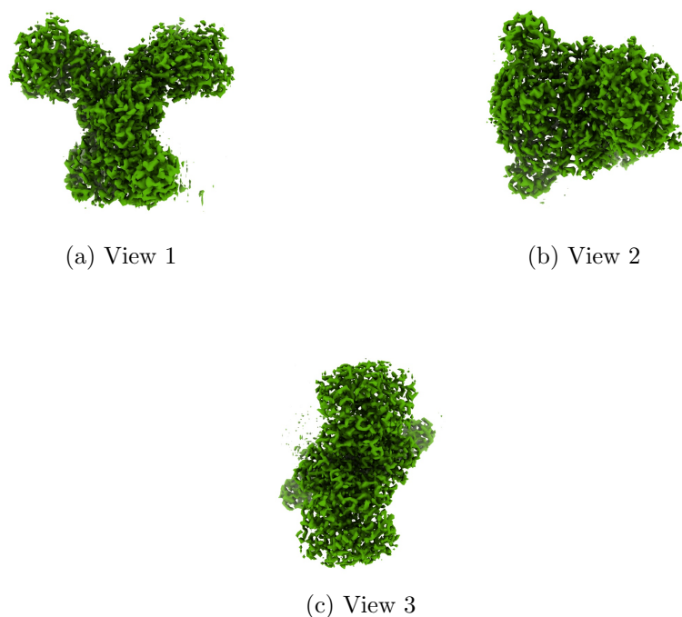
Figure 4: Isosurface at threshold=0.432000. Views generated by ChimeraX at a the following X, Y, Z angles: View 1 (0, -90, -90), View 2 (-90, 0, -90), View 3 (0, 0, 0).
