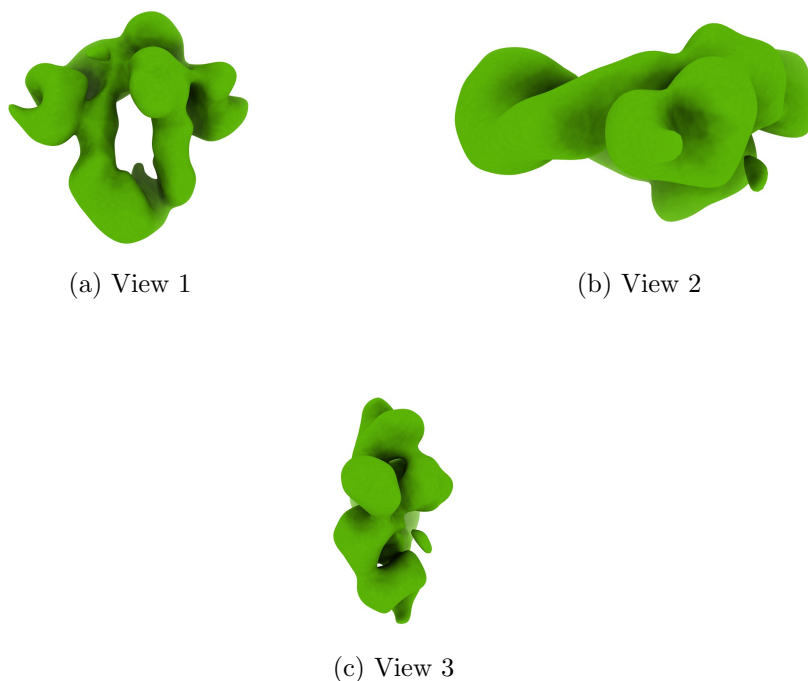
Figure 4: Isosurface at threshold=1.380000. Views generated by ChimeraX at a the following X, Y, Z angles: View 1 (0, -90, -90), View 2 (-90, 0, -90), View 3 (0, 0, 0).
