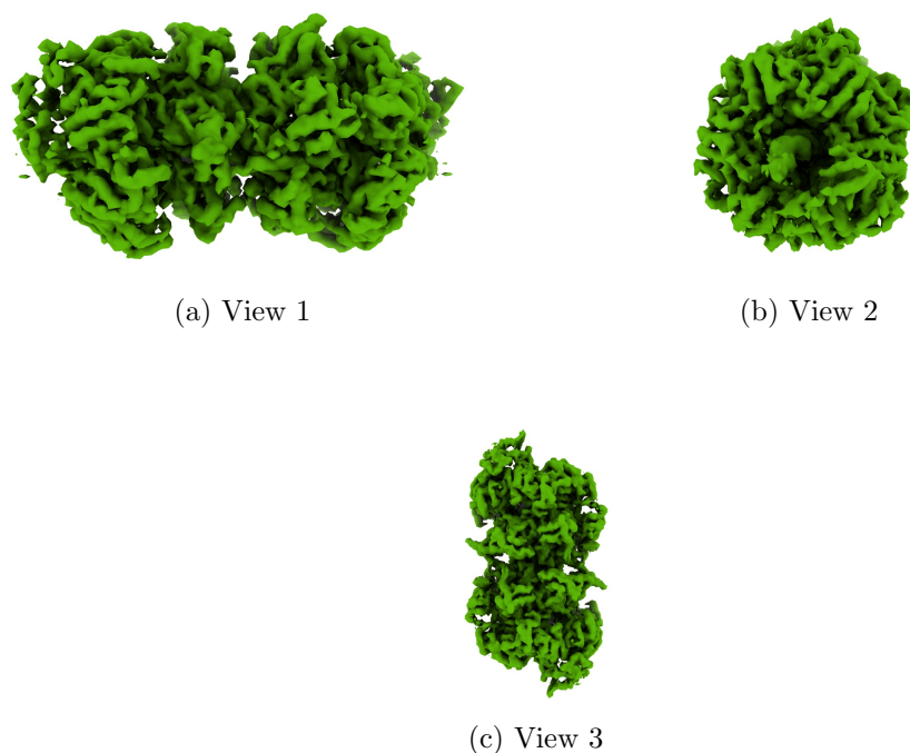
Figure 4: Isosurface at threshold=1.200000. Views generated by ChimeraX at a the following X, Y, Z angles: View 1 (0, -90, -90), View 2 (-90, 0, -90), View 3 (0, 0, 0).
