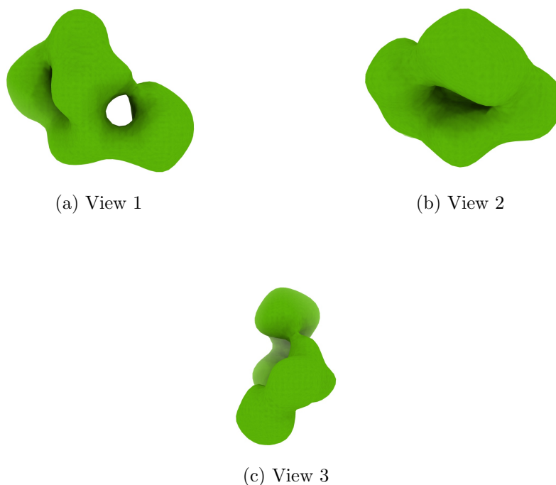
Figure 4: Isosurface at threshold=0.045000. Views generated by ChimeraX at a the following X, Y, Z angles: View 1 (0, -90, -90), View 2 (-90, 0, -90), View 3 (0, 0, 0).
