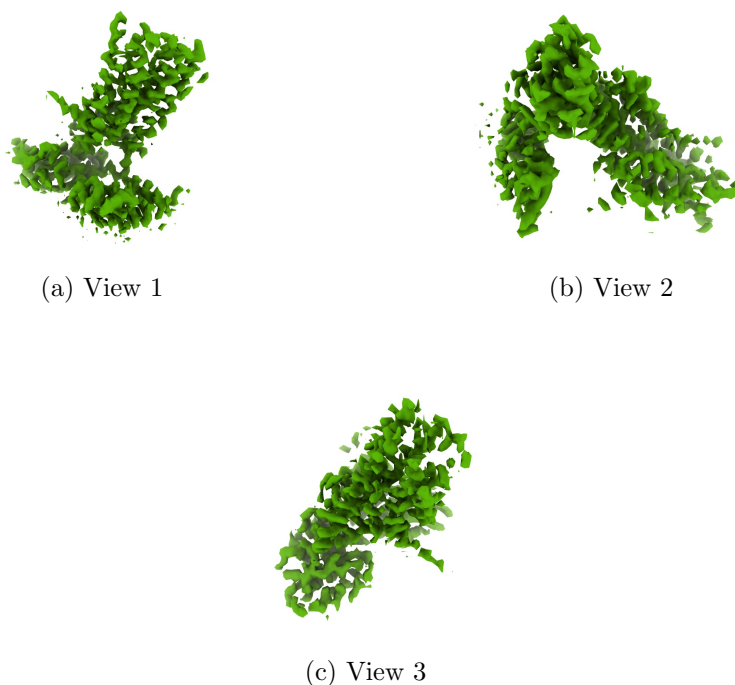
Figure 4: Isosurface at threshold=0.307000. Views generated by ChimeraX at a the following X, Y, Z angles: View 1 (0, -90, -90), View 2 (-90, 0, -90), View 3 (0, 0, 0).
