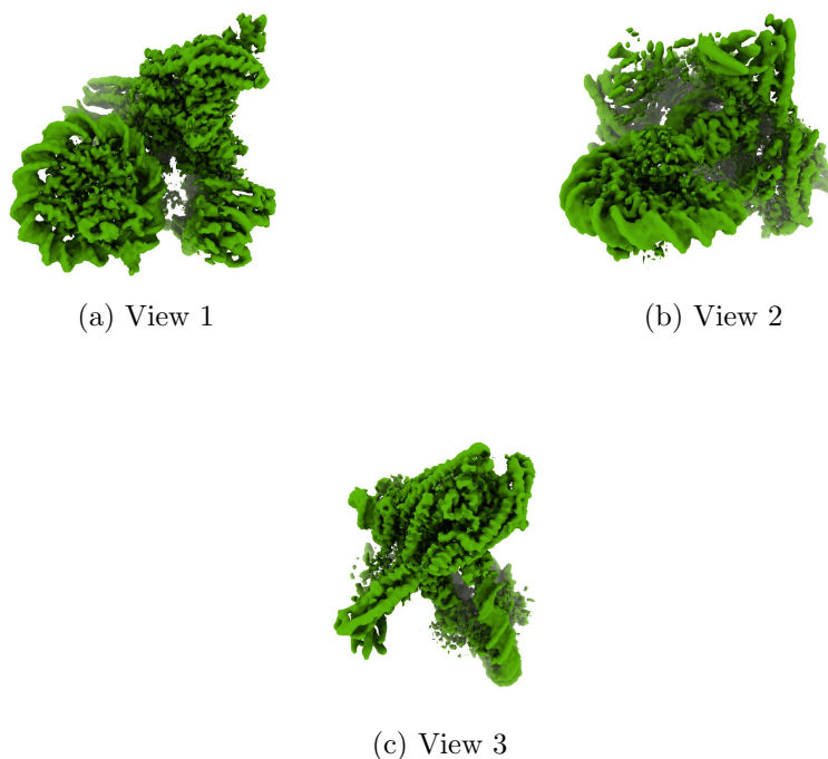
Figure 4: Isosurface at threshold=0.000200. Views generated by ChimeraX at a the following X, Y, Z angles: View 1 (0, -90, -90), View 2 (-90, 0, -90), View 3 (0, 0, 0).
