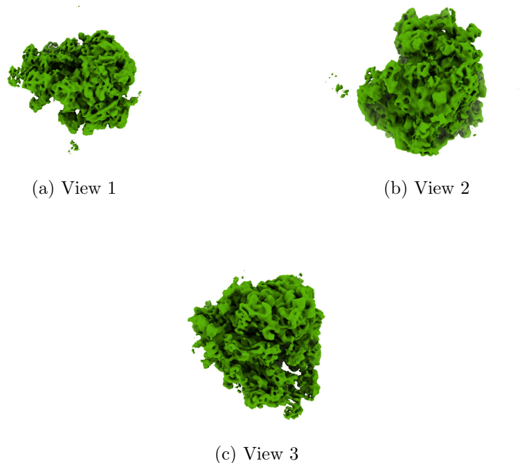
Figure 4: Isosurface at threshold=0.008540. Views generated by ChimeraX at a the following X, Y, Z angles: View 1 (0, -90, -90), View 2 (-90, 0, -90), View 3 (0, 0, 0).
