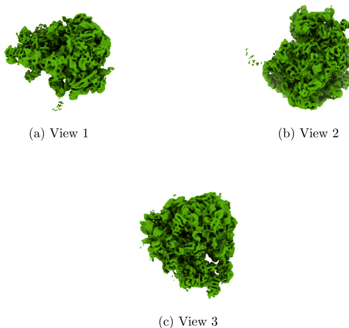
Figure 4: Isosurface at threshold=0.010900. Views generated by ChimeraX at a the following X, Y, Z angles: View 1 (0, -90, -90), View 2 (-90, 0, -90), View 3 (0, 0, 0).
