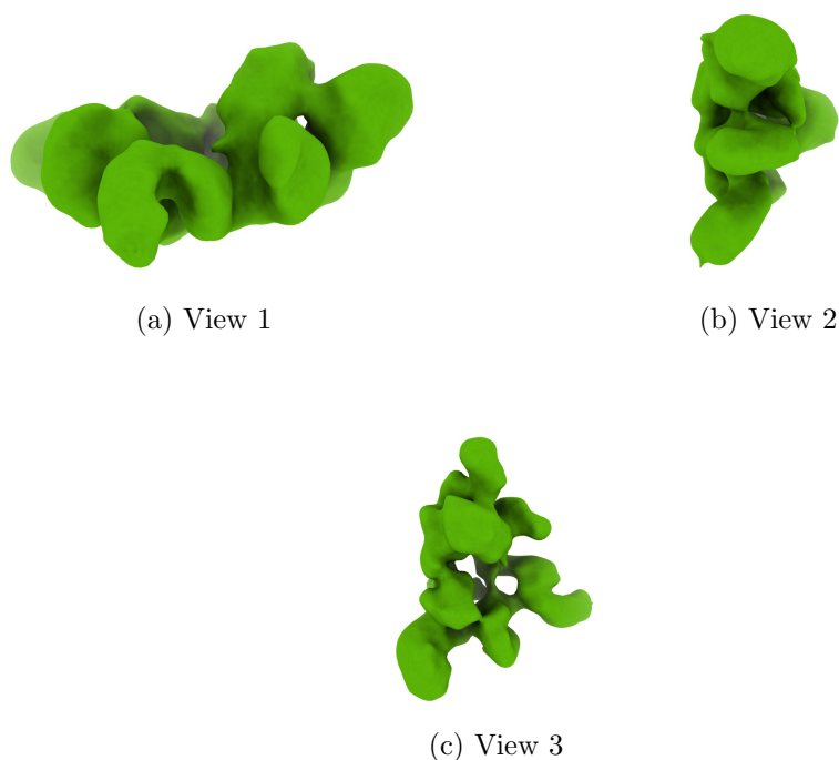
Figure 4: Isosurface at threshold=5.000000. Views generated by ChimeraX at a the following X, Y, Z angles: View 1 (0, -90, -90), View 2 (-90, 0, -90), View 3 (0, 0, 0).
