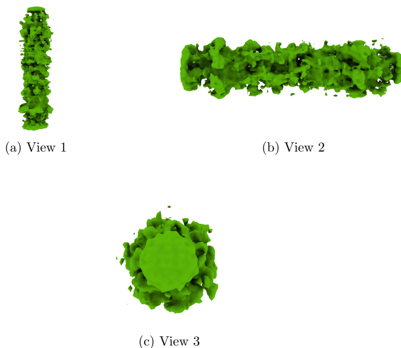
Figure 4: Isosurface at threshold=750.000000. Views generated by ChimeraX at a the following X, Y, Z angles: View 1 (0, -90, -90), View 2 (-90, 0, -90), View 3 (0, 0, 0).
