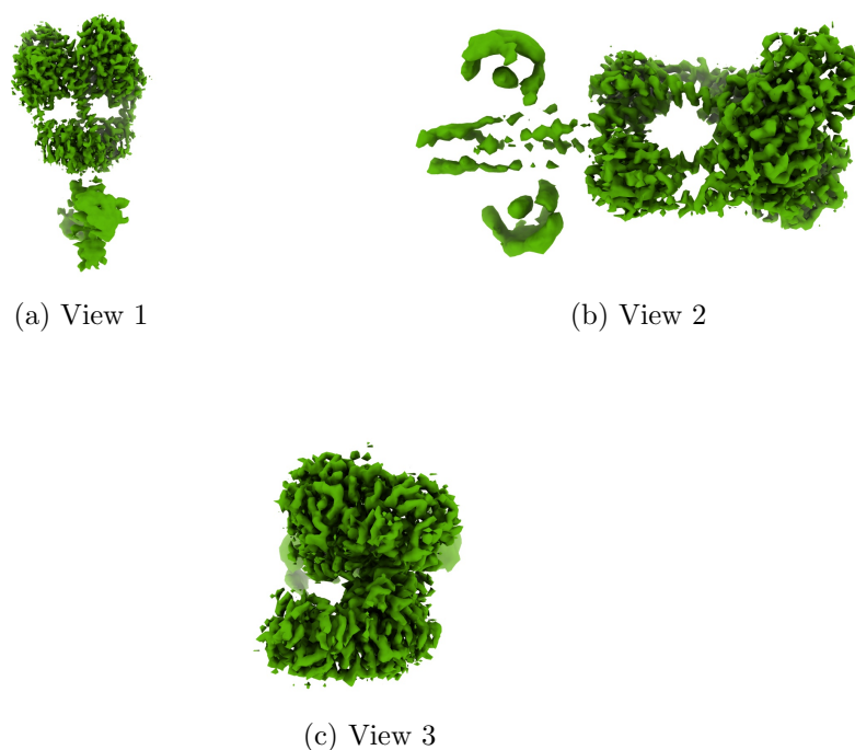
Figure 4: Isosurface at threshold=10.000000. Views generated by ChimeraX at a the following X, Y, Z angles: View 1 (0, -90, -90), View 2 (-90, 0, -90), View 3 (0, 0, 0).
