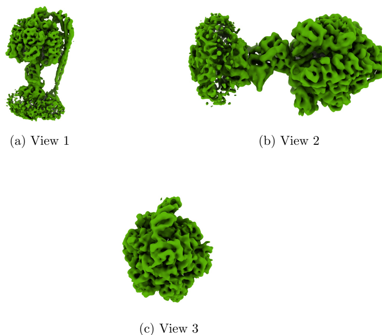
Figure 4: Isosurface at threshold=0.754000. Views generated by ChimeraX at a the following X, Y, Z angles: View 1 (0, -90, -90), View 2 (-90, 0, -90), View 3 (0, 0, 0).
