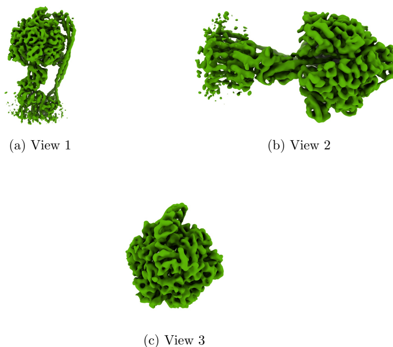
Figure 4: Isosurface at threshold=0.897000. Views generated by ChimeraX at a the following X, Y, Z angles: View 1 (0, -90, -90), View 2 (-90, 0, -90), View 3 (0, 0, 0).
