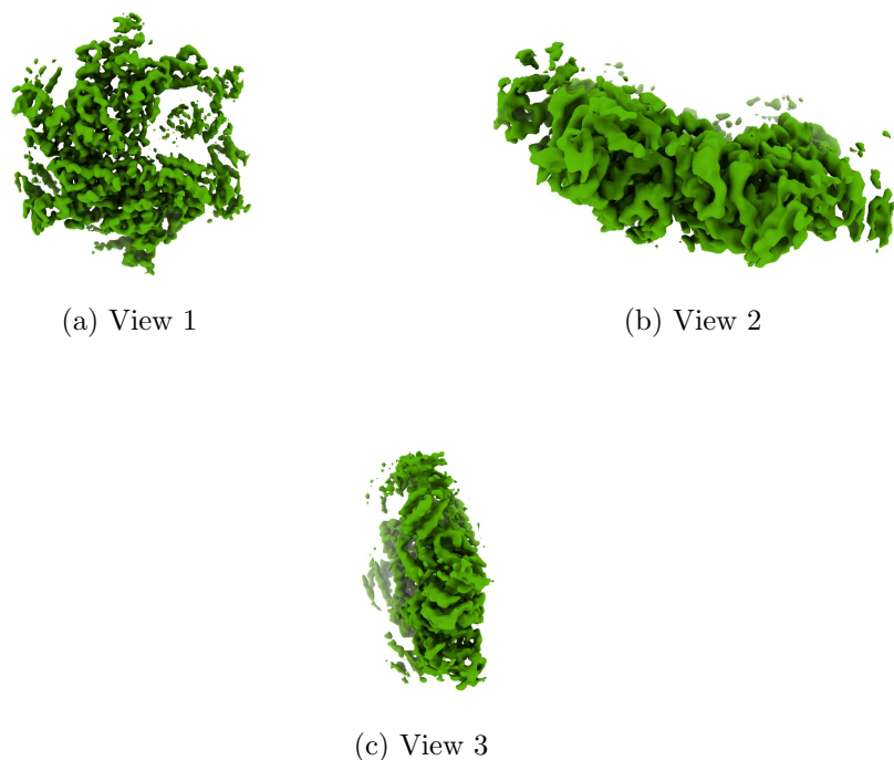
Figure 4: Isosurface at threshold=0.053800. Views generated by ChimeraX at a the following X, Y, Z angles: View 1 (0, -90, -90), View 2 (-90, 0, -90), View 3 (0, 0, 0).
