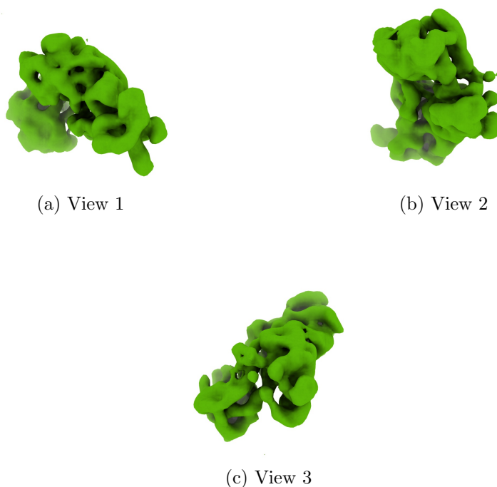
Figure 4: Isosurface at threshold=38.000000. Views generated by ChimeraX at a the following X, Y, Z angles: View 1 (0, -90, -90), View 2 (-90, 0, -90), View 3 (0, 0, 0).
