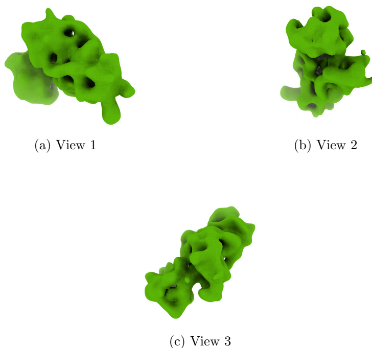
Figure 4: Isosurface at threshold=32.000000. Views generated by ChimeraX at a the following X, Y, Z angles: View 1 (0, -90, -90), View 2 (-90, 0, -90), View 3 (0, 0, 0).
