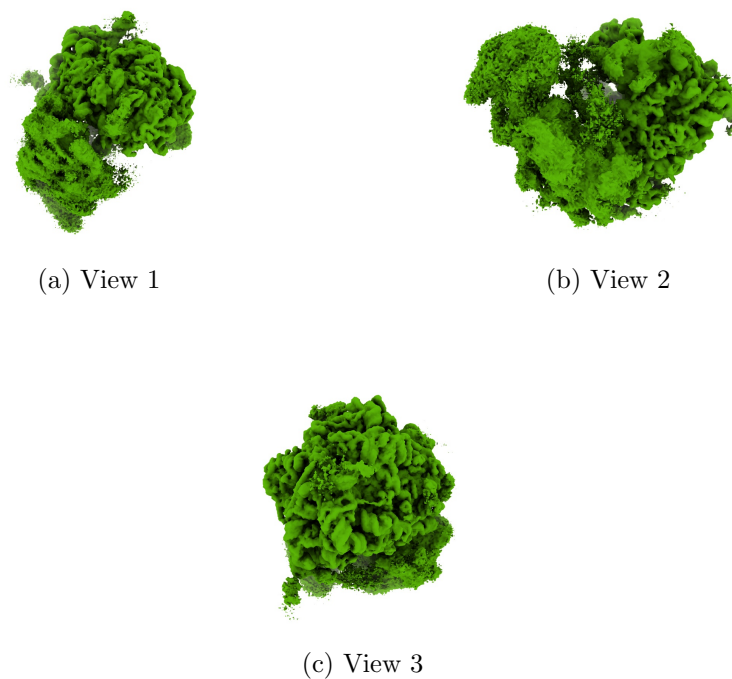
Figure 4: Isosurface at threshold=0.006700. Views generated by ChimeraX at a the following X, Y, Z angles: View 1 (0, -90, -90), View 2 (-90, 0, -90), View 3 (0, 0, 0).
