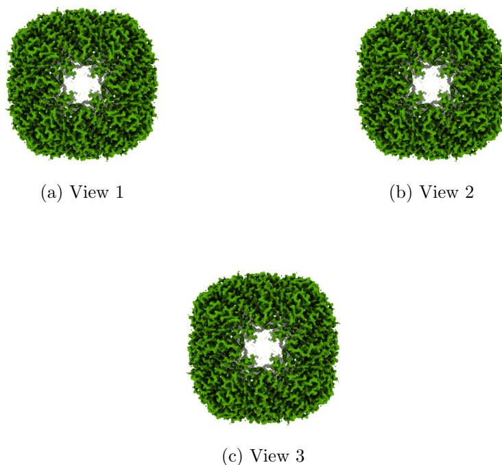
Figure 4: Isosurface at threshold=78.000000. Views generated by ChimeraX at a the following X, Y, Z angles: View 1 (0, -90, -90), View 2 (-90, 0, -90), View 3 (0, 0, 0).
