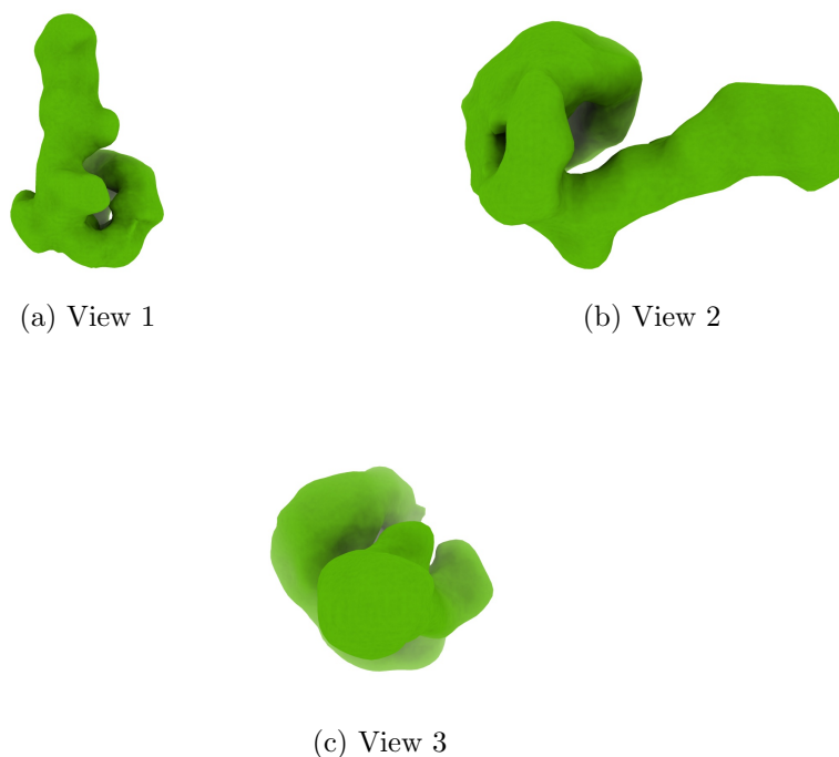
Figure 4: Isosurface at threshold=5.500000. Views generated by ChimeraX at a the following X, Y, Z angles: View 1 (0, -90, -90), View 2 (-90, 0, -90), View 3 (0, 0, 0).
