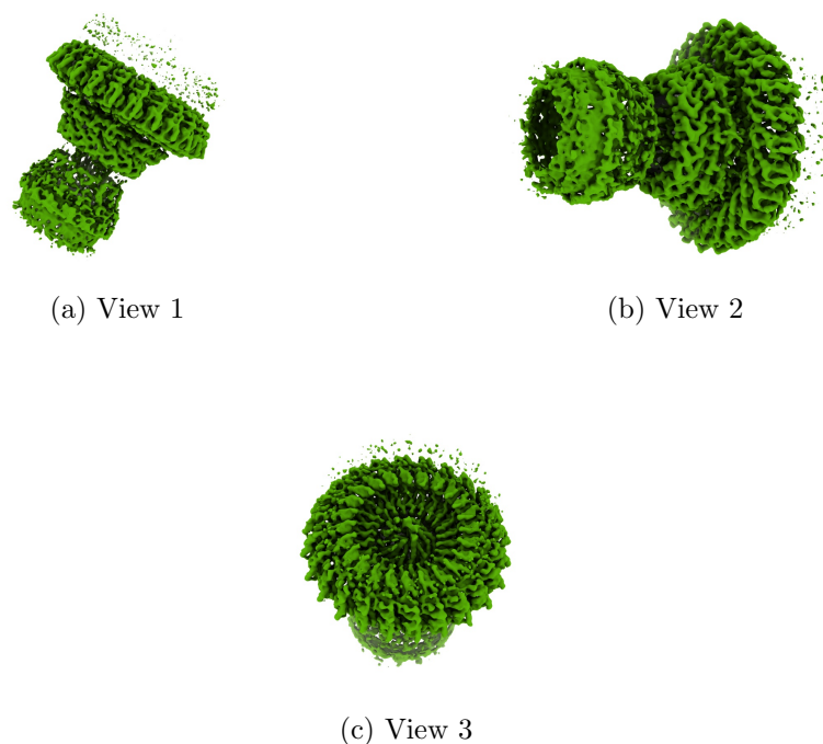
Figure 4: Isosurface at threshold=0.027000. Views generated by ChimeraX at a the following X, Y, Z angles: View 1 (0, -90, -90), View 2 (-90, 0, -90), View 3 (0, 0, 0).
