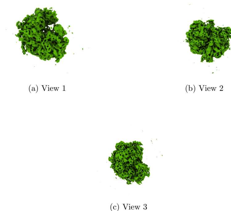
Figure 4: Isosurface at threshold=0.048000. Views generated by ChimeraX at a the following X, Y, Z angles: View 1 (0, -90, -90), View 2 (-90, 0, -90), View 3 (0, 0, 0).
