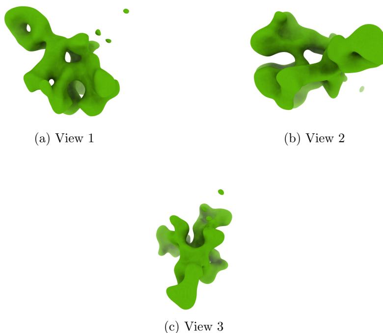
Figure 4: Isosurface at threshold=0.022900. Views generated by ChimeraX at a the following X, Y, Z angles: View 1 (0, -90, -90), View 2 (-90, 0, -90), View 3 (0, 0, 0).
