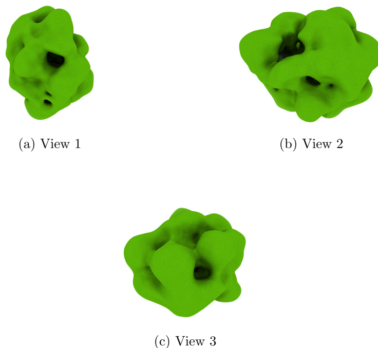
Figure 4: Isosurface at threshold=0.042200. Views generated by ChimeraX at a the following X, Y, Z angles: View 1 (0, -90, -90), View 2 (-90, 0, -90), View 3 (0, 0, 0).
