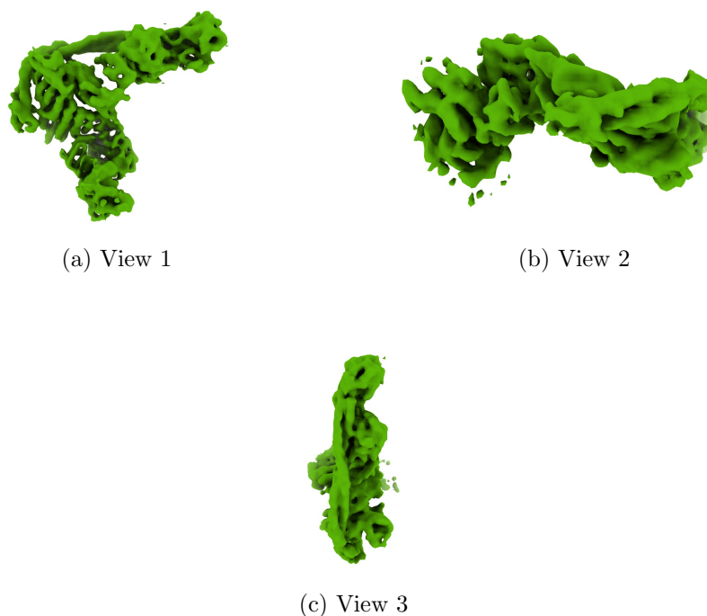
Figure 4: Isosurface at threshold=0.012700. Views generated by ChimeraX at a the following X, Y, Z angles: View 1 (0, -90, -90), View 2 (-90, 0, -90), View 3 (0, 0, 0).
