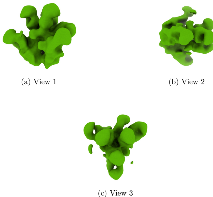
Figure 4: Isosurface at threshold=0.011300. Views generated by ChimeraX at a the following X, Y, Z angles: View 1 (0, -90, -90), View 2 (-90, 0, -90), View 3 (0, 0, 0).
