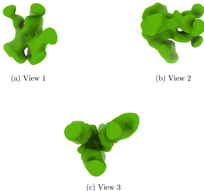
Figure 4: Isosurface at threshold=0.024700. Views generated by ChimeraX at a the following X, Y, Z angles: View 1 (0, -90, -90), View 2 (-90, 0, -90), View 3 (0, 0, 0).
