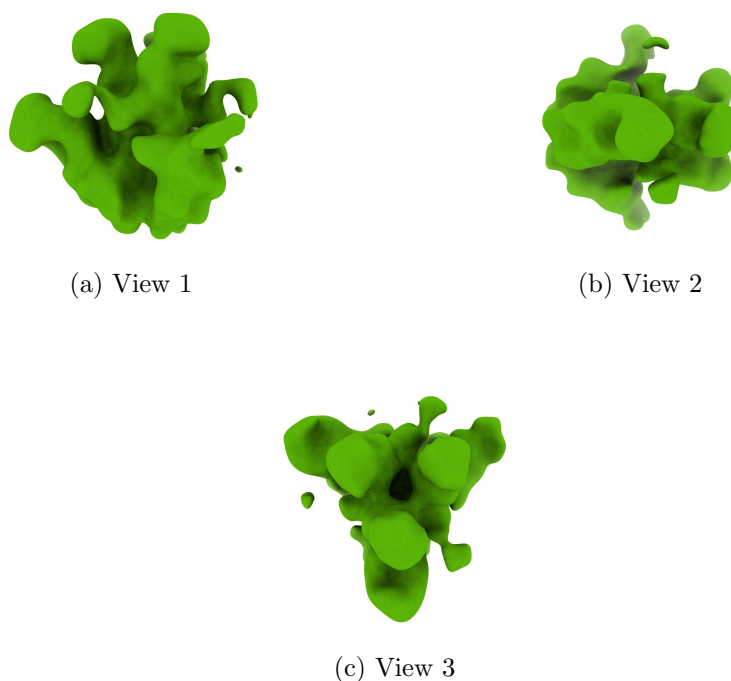
Figure 4: Isosurface at threshold=0.007700. Views generated by ChimeraX at a the following X, Y, Z angles: View 1 (0, -90, -90), View 2 (-90, 0, -90), View 3 (0, 0, 0).
