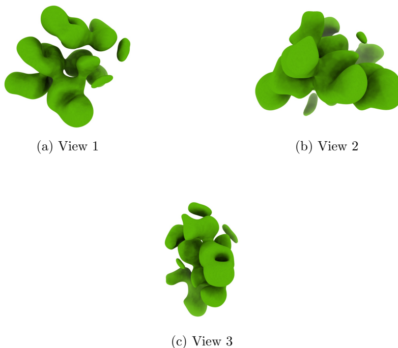
Figure 4: Isosurface at threshold=0.810000. Views generated by ChimeraX at a the following X, Y, Z angles: View 1 (0, -90, -90), View 2 (-90, 0, -90), View 3 (0, 0, 0).
