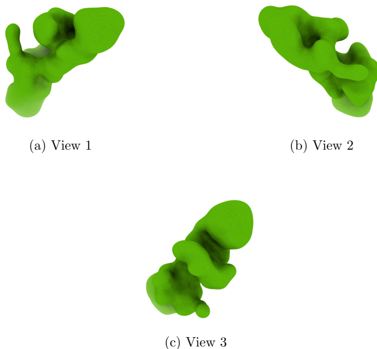
Figure 4: Isosurface at threshold=2.520000. Views generated by ChimeraX at a the following X, Y, Z angles: View 1 (0, -90, -90), View 2 (-90, 0, -90), View 3 (0, 0, 0).
