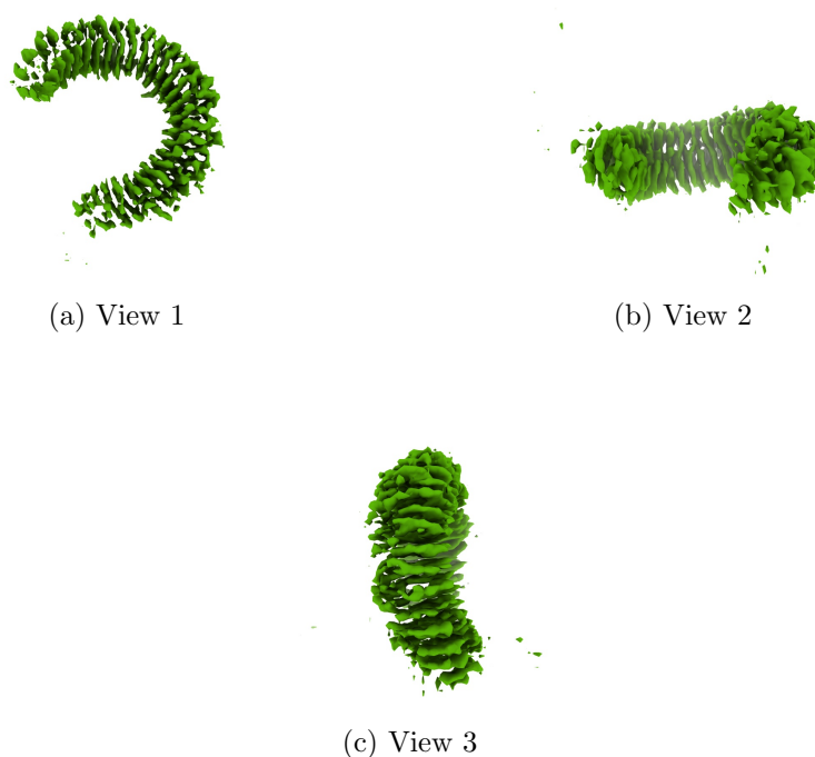
Figure 4: Isosurface at threshold=0.530000. Views generated by ChimeraX at a the following X, Y, Z angles: View 1 (0, -90, -90), View 2 (-90, 0, -90), View 3 (0, 0, 0).
