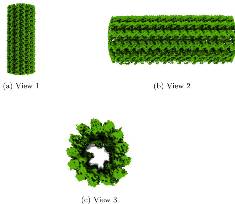
Figure 4: Isosurface at threshold=12.000000. Views generated by ChimeraX at a the following X, Y, Z angles: View 1 (0, -90, -90), View 2 (-90, 0, -90), View 3 (0, 0, 0).
