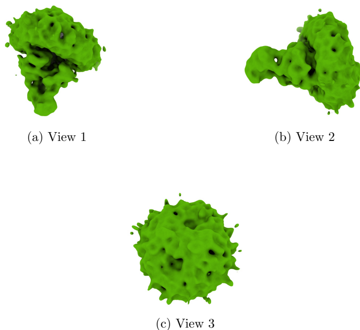
Figure 4: Isosurface at threshold=0.391000. Views generated by ChimeraX at a the following X, Y, Z angles: View 1 (0, -90, -90), View 2 (-90, 0, -90), View 3 (0, 0, 0).
