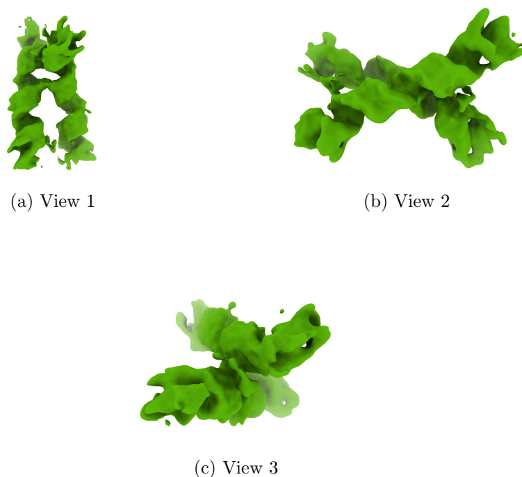
Figure 4: Isosurface at threshold=0.601000. Views generated by ChimeraX at a the following X, Y, Z angles: View 1 (0, -90, -90), View 2 (-90, 0, -90), View 3 (0, 0, 0).
