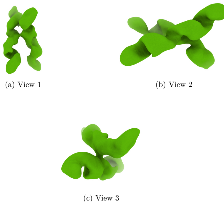
Figure 4: Isosurface at threshold=0.470000. Views generated by ChimeraX at a the following X, Y, Z angles: View 1 (0, -90, -90), View 2 (-90, 0, -90), View 3 (0, 0, 0).
