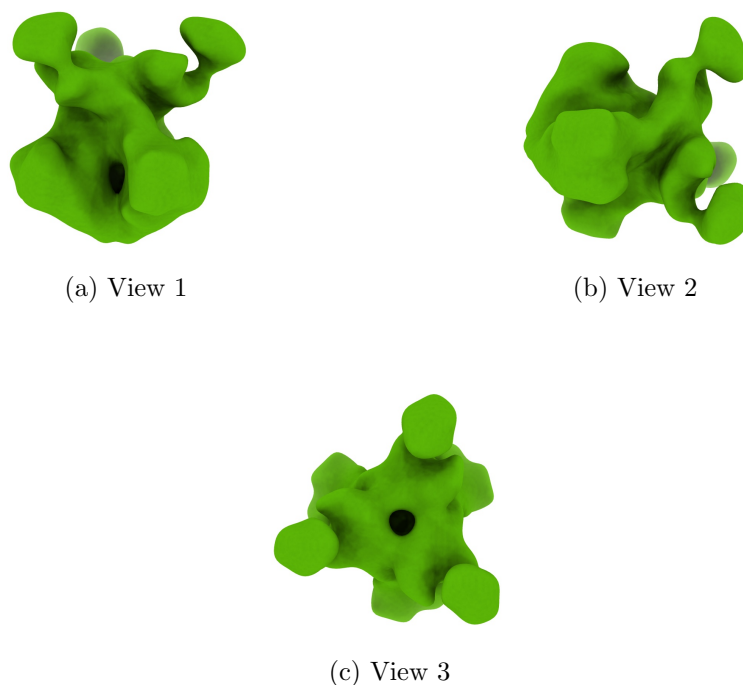
Figure 4: Isosurface at threshold=0.530000. Views generated by ChimeraX at a the following X, Y, Z angles: View 1 (0, -90, -90), View 2 (-90, 0, -90), View 3 (0, 0, 0).
